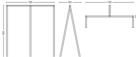
LOOP STAND WARDROBE WIDTH 130 CM DEPTH 60 CM HEIGHT 150 CM
