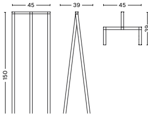
LOOP STAND HALL WIDTH 45 CM DEPTH 39 CM HEIGHT 150 CM
